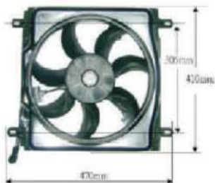
COOLING FAN SIZE: 470mm x 410mm 24V, 2723 RPM, 7-BLADE, 8.8A, 211.2W
